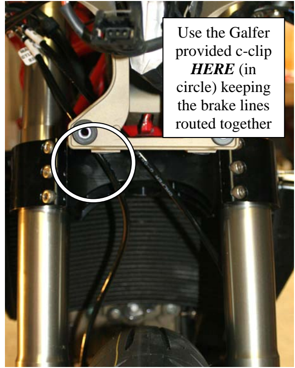
b. Routing in front of lower triple tree
