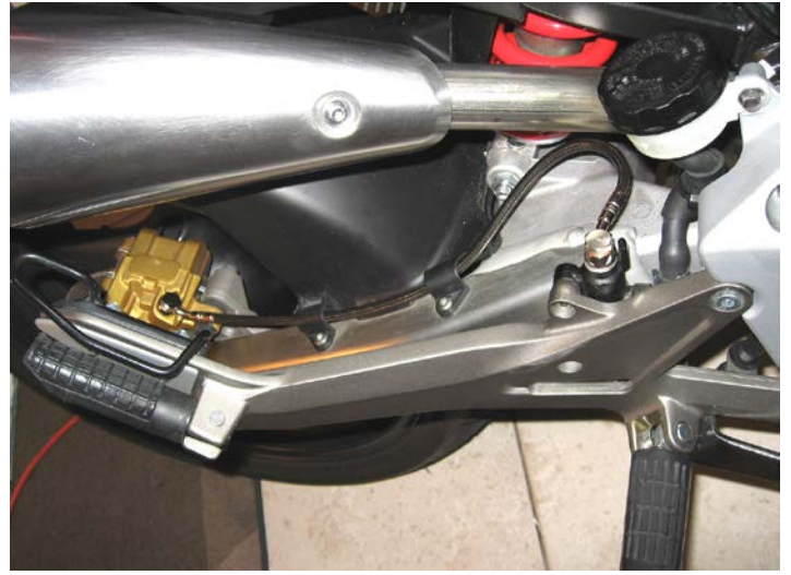
b. Rear line overall, using OEM tabs for routing purposes
